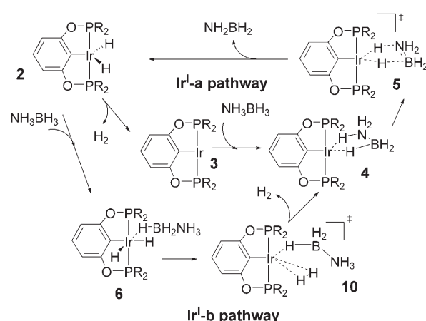
Scheme 1. Dehydrogenation pathways IrI-a (2–3–4–5–2) and IrI-b (2–6–10–4–5–2) for AB dehydrogenation. R = methyl.
